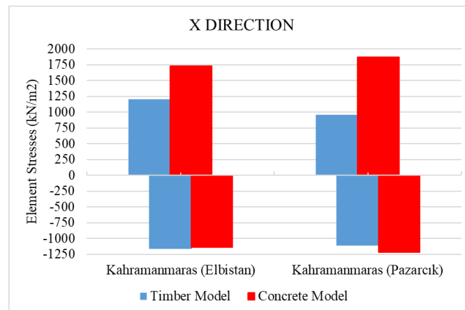
Figure 11. Element stress values of models in x directions
