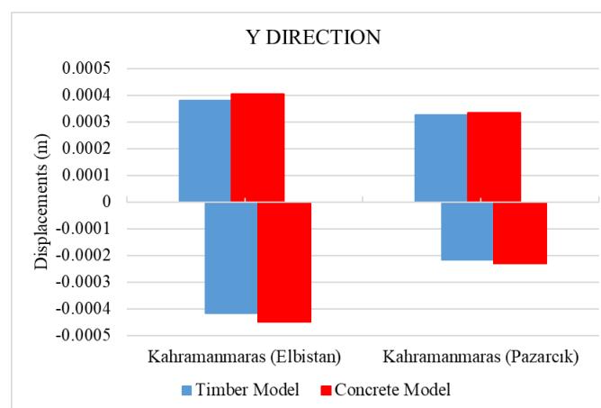
Figure 10. Displacement values of models in y directions
