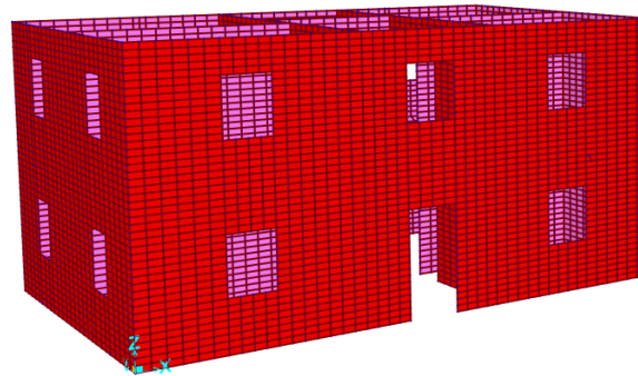
Figure 2. Finite element model of historical building
