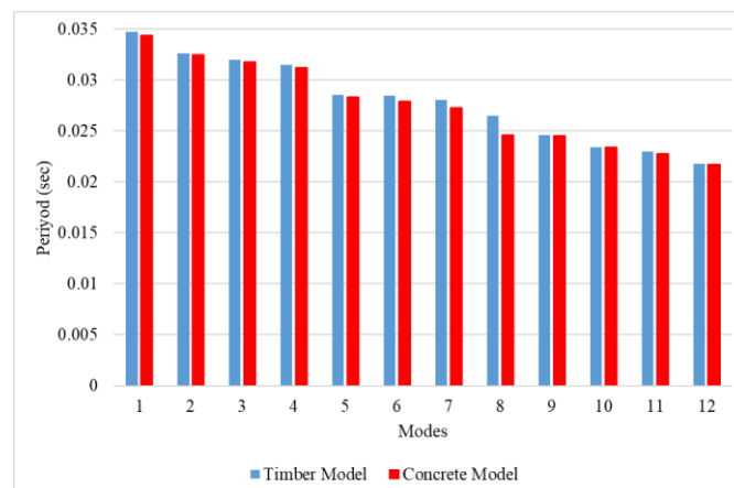
Figure 6. The period values of the structures
