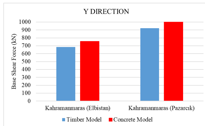
Figure 8. Base Shear Force in Y direction for models in y directions
