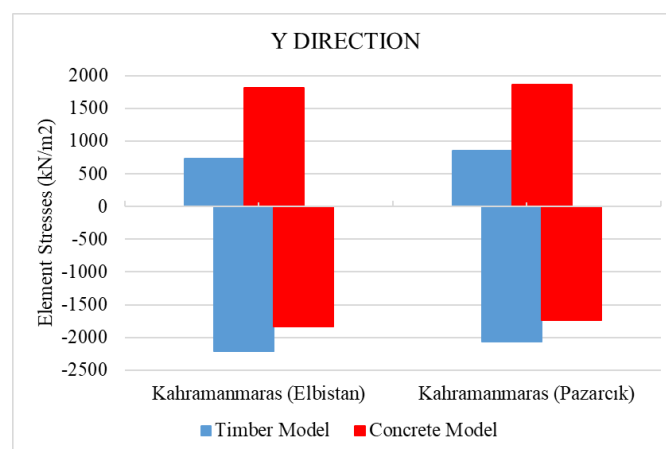
Figure 12. Element stress values of models in y directions
