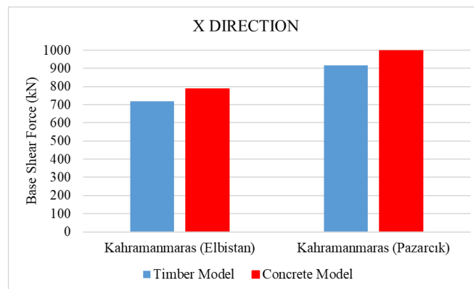
Figure 7. Base Shear Force in X direction for models in x directions
