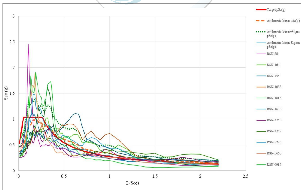
Figure 2. Spectrums of earthquakes
