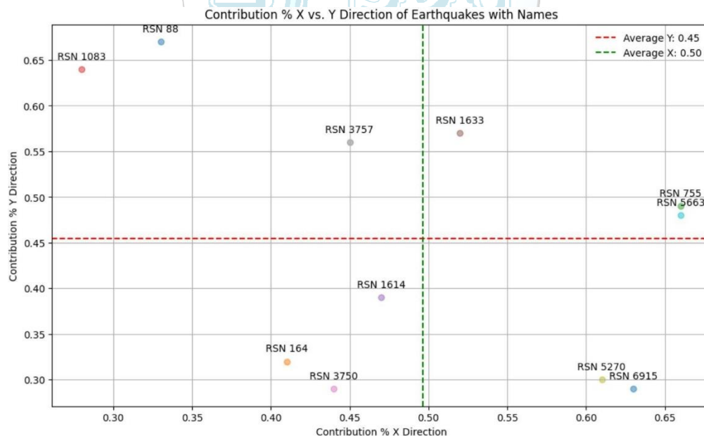
Figure 7. X% and Y Direction Contribution of the Timber model with the names of the earthquakes
