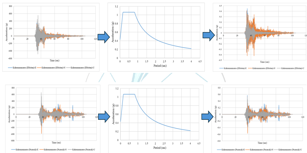
Figure 5. Scaling of acceleration time graphs
