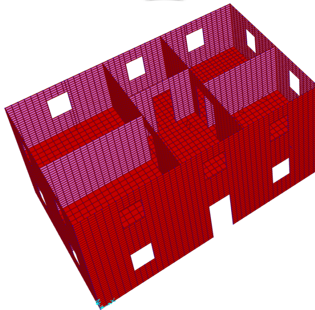
Figure 4. Concrete slab model
