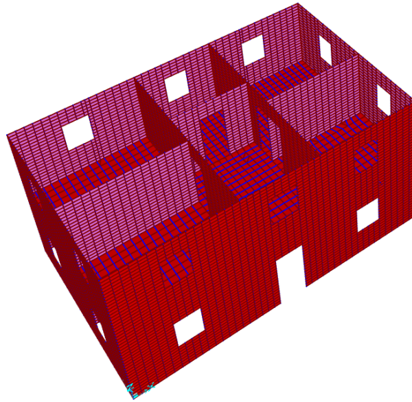
Figure 3. Timber slab model
