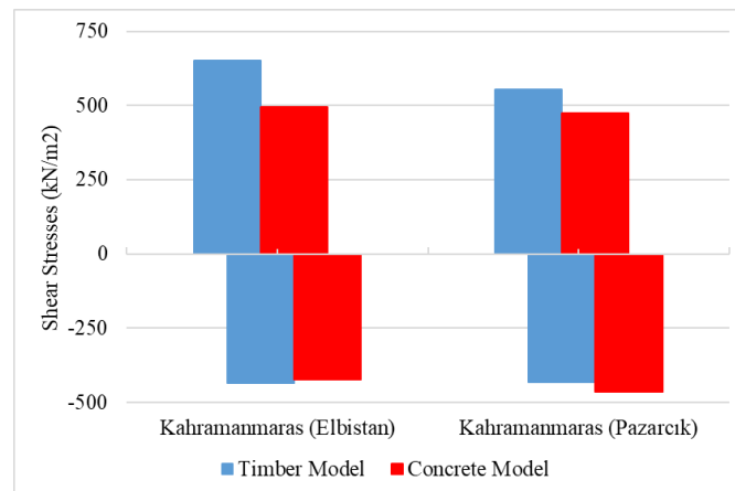
Figure 13. Shear stress values of models
