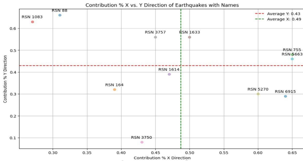
Figure 6. X% and Y Direction Contribution of the Aluminum model with the names of the earthquakes
